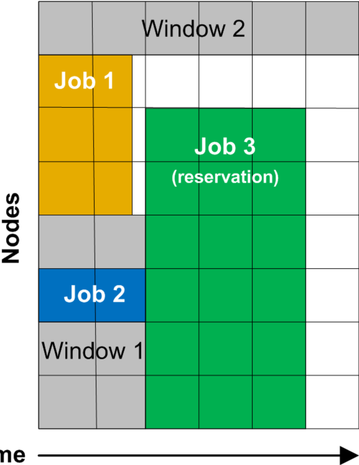
Image 7-1: Backfillable nodes create backfill windows 1 and 2
