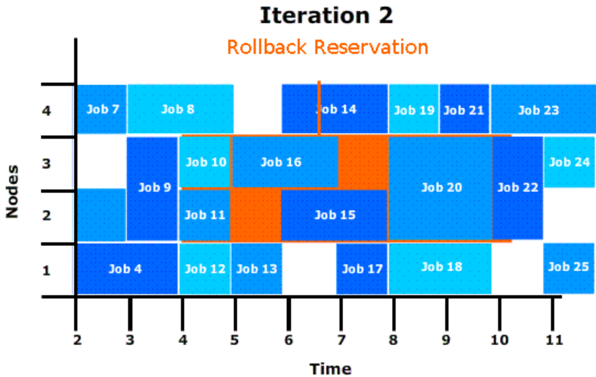
Image 6-3: Rollback reservation Iteration 2
